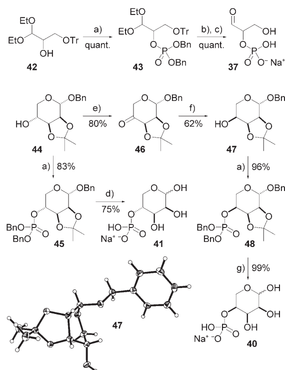
Scheme 9. Conventional synthesis of rac -glyceraldehyde-2-phosphate 37 , L-ribose-4-phosphate 40 and D-lyxose-4-phosphate 41 . a) t BuOK, THF, RT → -40 °C, (BnO) 2 P(O)OP(O)(OBn) 2 ; b) H 2 , Pd/C, dioxane/H 2 O; c) D 2 O, pD ≈ 2.2, 50 °C, 2 d then H 2 O pH → 7 (NaOH aq.); d) H 2 , Pd/C, MeOH then pH → 1 (HCl aq.), 40 °C, 3 h then pH → 7 (NaOH aq.); e) CrO 3 , py, Ac 2 O, CH 2 Cl 2 ; f) NaBH 4 , EtOH, 0 °C; g) H 2 , Pd/C, MeOH then pH → 7 (NaOH aq.).
