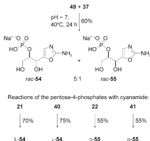
Scheme 11. Formation of pentose-aminooxazole-4'-phosphates.
