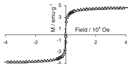
Figure 2. Field-dependent magnetization curve for \text{Fe}_x\text{O}_y @Ti-HMS measured at 300 K.
