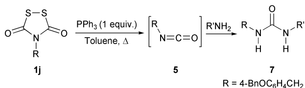
Scheme 7 Urea formation.
