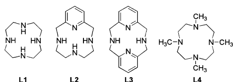
Figure 1. Macroscopic polyamine (MCPA) ligands studied here.
