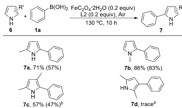
Scheme 1. Iron-Catalyzed Arylation of Substituted Pyrroles with Phenylboronic Acid a,b
