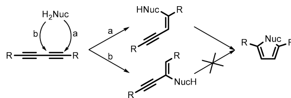
Scheme 2. Regioselectivity of the First Addition Step
