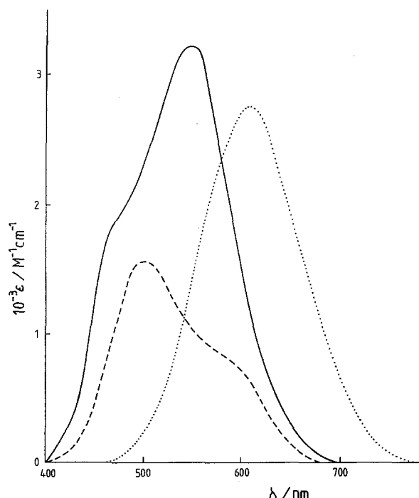
Fig. 1. Electronic spectra of cysteine complexes of iron(III) scaled to indicate relative molar absorptions. \text{FeL}^+ : ...( \text{pH} 2.7–4.5); \text{Fe(OH)L} : ...( \text{pH} 5.1–6.7); \text{Fe(OH)L}_2^{2-} : ...( \text{pH} 8.6–11.6)
