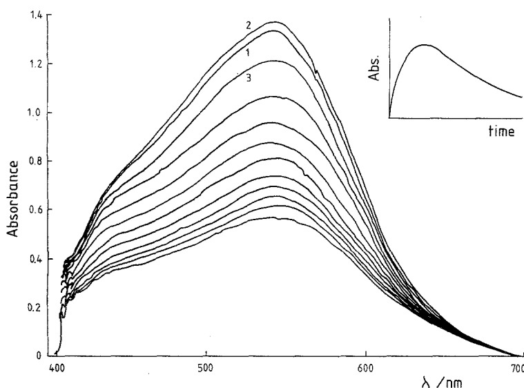
Fig. 8. Kinetic run for the formation and decay of \text{Fe}(\text{OH})\text{L}_2^{2-} showing constancy of the spectra obtained (insert shows envelope; pH=9.58 ; time interval = 9 999 ms)
