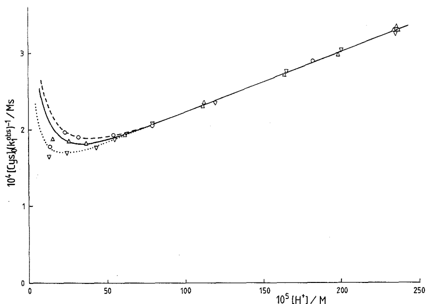
Fig. 4. Dependence of [\text{Cys}]_0/k_2^{\text{obs}} ( = 1/k_2' ) for the decomposition of \text{FeL}^+ on [\text{H}^+] . At low [\text{H}^+] values the single line divides into separate curves according to the [\text{Cys}]_0 value. The theoretical curves are calculated for \log K_1^M = 13.70 (see text) with: [\text{Cys}]_0 = 0.0125 \text{ M} --○--; 0.01 \text{ M} —△—; 0.005 \text{ M} ...▽...
