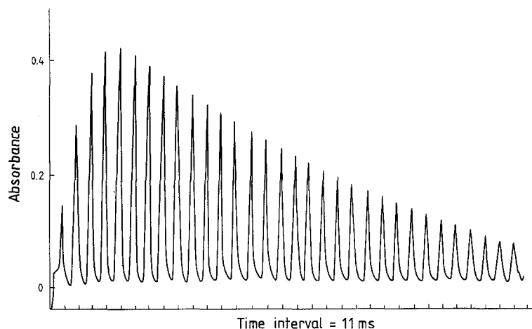
Fig. 2. Kinetic run recorded as a set of sequential complete spectra (spectral scan = 405–960 nm) taken at a scan rate of 11 ms/spectrum ( \text{pH} = 2.97)
