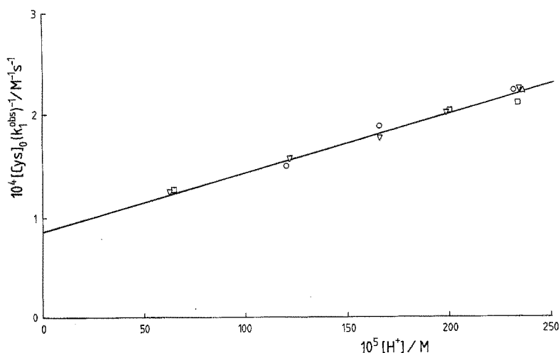
Fig. 3. Dependence of [\text{Cys}]_0/k_1^{\text{obs}} (= 1/k_1') for the formation of \text{FeL}^+ on [\text{H}^+] for two [\text{Cys}]_0 values: i) [\text{Cys}]_0 = 0.01 \text{ M} : [\text{Fe}]_0 = 0.001 \text{ M} (o), 0.0005 \text{ M} ( \Delta ), 0.00025 \text{ M} ( \nabla ) and ii) [\text{Cys}]_0 = 0.005 \text{ M} : [\text{Fe}]_0 = 0.001 \text{ M} ( \square )
