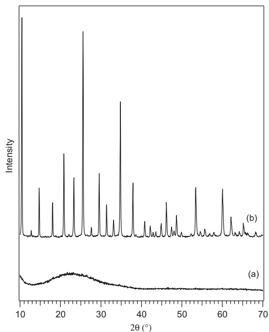
Fig. 4. The high angle XRD patterns of (a) 10 wt.% TPA/MCM-41, (b) TPA.
