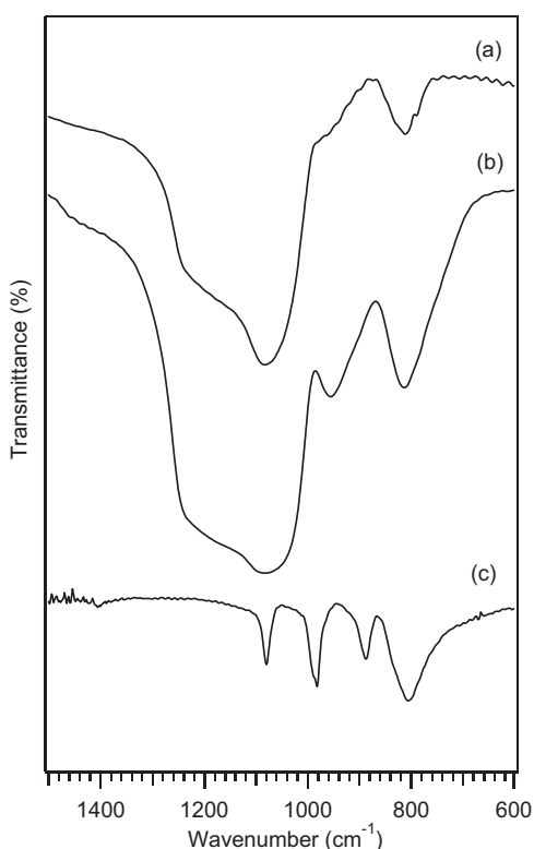
Fig. 2. FT-IR spectra of (a) MCM-41; (b) 10 wt.% TPA/MCM-41, (c) pure TPA.
