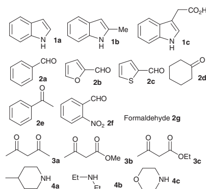
Scheme 3. Various substrates.
