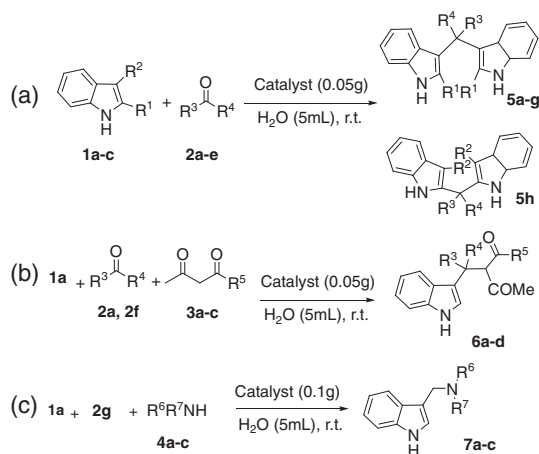
Scheme 4. Various reactions for the synthesis of indole derivatives.
