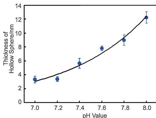
Figure 5. Relationship for the thickness of the SiO 2 capsules with pH values used for the preparation of PS-PEI templates.
