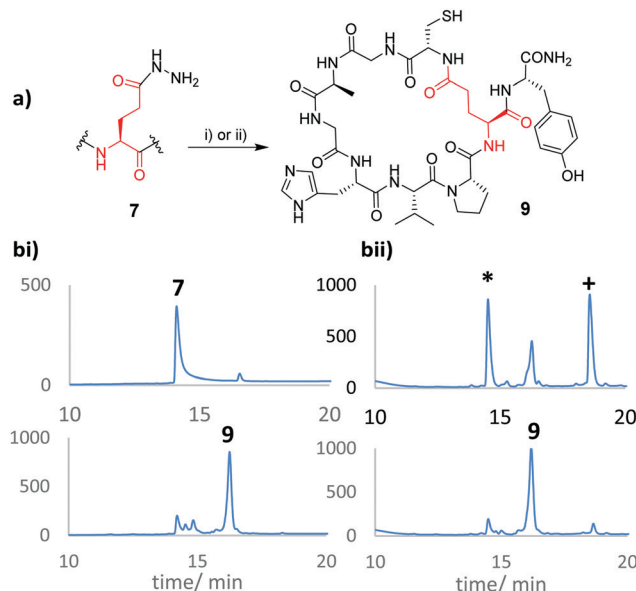
Fig. 2 (a) Acyl hydrazide activation to form macrocycle 9 , monitored by HPLC. (bi) Upper trace shows initial hydrazide 7 while the lower trace shows the reaction mixture after NaNO 2 activation (20 min at pH3, 0 °C), followed by addition of sodium 2-mercaptoethane sulfonate (MESNa), 1 h, RT, pH 7. 3c (bii) Activation of 7 with acetyl acetone (acac)/MESNa (pH 3–4, 2 h, upper trace) leads to a mix of MESNa thioester (*) and acyl pyrazole (+) which are both consumed upon adjusting to pH7 for 1 h (lower trace). 12
