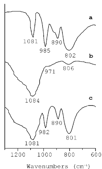
Figure 3. FT-IR spectrum of a) bulk TPA, b) SBA-15, and c) \text{TPA}_{60}/\text{SBA-15v} .
