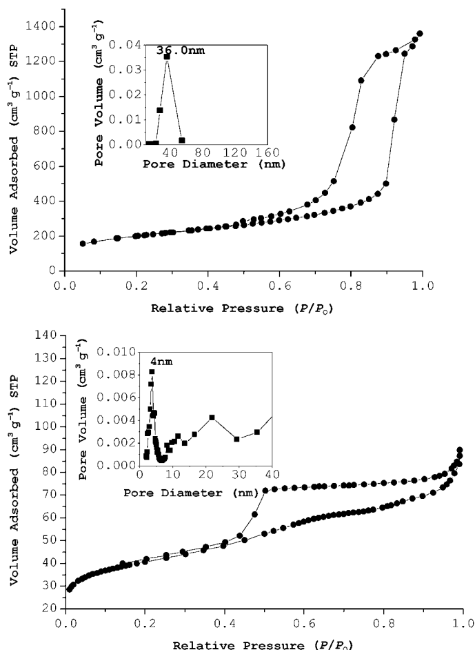
Figure 1. Nitrogen adsorption–desorption isotherm plots and pore size distribution curve for SBA-15 (top) and \text{TPA}_{60}/\text{SBA-15v} (bottom).
