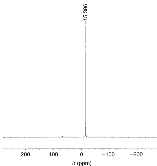
Figure 2. ^{31}\text{P} NMR MAS spectrum of \text{TPA}_{60}/\text{SBA-15v} .
