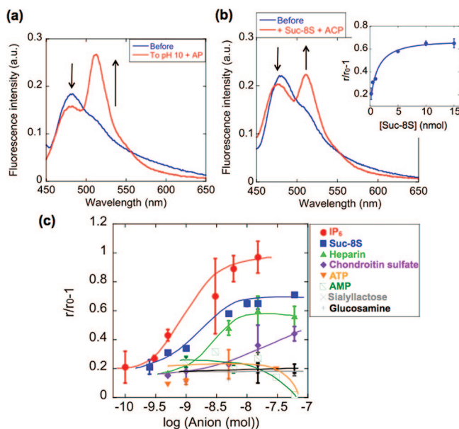
Figure 8. Fluorescence spectral changes ( \lambda_{\text{ex}} = 429 nm) of hydrogel 1 containing BODIPY 4 and P-coum 3 encapsulated \text{NH}_2 -MCM (a) before and after adjusting to pH 10 and AP addition and (b) before and after Suc-8S and ACP addition. The inset in (b) shows the fluorescence titration curve for Suc-8S ( [\text{Suc-8S}] = 0\text{--}1.4 mM ( 0\text{--}15 nmol)). Conditions: [1] = 0.090 wt % (50 mM Tris-HCl buffer, pH 5.0, [4] = 2.0 \mu\text{M} for (a) and 200 mM acetate buffer, pH 5.0, [4] = 3.0 \mu\text{M} , [\text{Suc-8S}] = 1.4 mM (15 nmol) for (b)), [\text{P-coum } \mathbf{3}@\text{NH}_2\text{-MCM}] = 5.0 mg \text{mL}^{-1} (50 \mu\text{g} ), RT. (c) Plots of the relative fluorescence intensity changes ( r/r_0 - 1 = (F_{513}/F_{483})/(F_{513}/F_{483})_0 - 1 ) of hydrogel 1 containing BODIPY 4 and P-coum 3 encapsulated \text{NH}_2 -MCM upon addition of various species and ACP ( \lambda_{\text{ex}} = 429 nm). Conditions: [1] = 0.090 wt % (200 mM acetate buffer, pH 5.0), [4] = 3.0 \mu\text{M} , [\text{anion}] = 0\text{--}6.5 mM ( 0\text{--}60 nmol), [\text{P-coum } \mathbf{3}@\text{NH}_2\text{-MCM}] = 5.0 mg \text{mL}^{-1} (50 \mu\text{g} ), RT.
