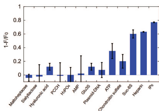
Figure 5. Changes in fluorescence intensity ratio of the hydrogel 1 droplet containing P-coum 2 encapsulated NH 2 –MCM upon the addition of anionic species. Conditions: [ 1 ] = 0.090 wt % (200 mM acetate buffer, pH 5.0), [anion] = 1.0 mM (0.50 nmol), [P-coum 2 @NH 2 –MCM] = 0.83 mg mL −1 (0.80 \mu\text{g} ), RT.
