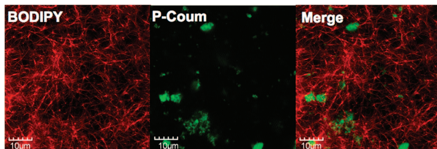
Figure 3. CLSM images of the hydrogel 1 droplet containing BODIPY 4 and P-coum 2 encapsulated NH 2 –MCM. The left image shows the localization of BODIPY 4 ( \lambda_{\text{ex}} = 488 \text{ nm}/\lambda_{\text{em}} = 515\text{--}570 \text{ nm} ), the middle image shows the localization of P-coum 2 ( \lambda_{\text{ex}} = 458 \text{ nm}/\lambda_{\text{em}} = 470\text{--}510 \text{ nm} ), and the merge image shown in the right panel was obtained by summing the left and middle images. Conditions: [ 1 ] = 0.090 wt % (50 mM Tris-HCl buffer, pH 5.0), [ 4 ] = 5.0 \mu\text{M} , [P-coum 2 @NH 2 –MCM] = 9.0 mg mL −1 (4.5 \mu\text{g} ), RT.
