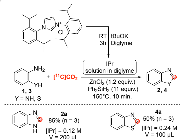
Scheme 4. Cyclization reactions with home-made solution of IPr . Radiochemical yields are mean values and were estimated from trapped [^{11}\text{C}]\text{CO}_2 within the reactor and are decay-corrected from end of [^{11}\text{C}]\text{CO}_2 trapping inside reactor.
