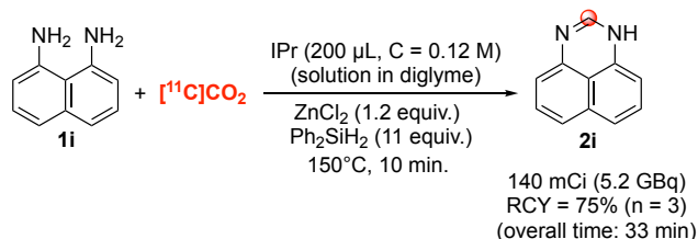
Scheme 5. Production of perimidine 2i . The RCY value is mean value and was estimated from trapped [^{11}\text{C}]\text{CO}_2 within the reactor and are decay-corrected from end of [^{11}\text{C}]\text{CO}_2 trapping inside reactor.
