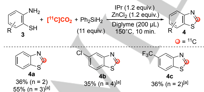
Scheme 2. Cyclizations of aminobenzenethiols with [^{11}\text{C}]\text{CO}_2 . Radiochemical yields are mean values and were estimated from trapped [^{11}\text{C}]\text{CO}_2 within the reactor and are decay-corrected from end of [^{11}\text{C}]\text{CO}_2 trapping inside reactor. [a] diglyme volume = 100 \mu\text{L} .
