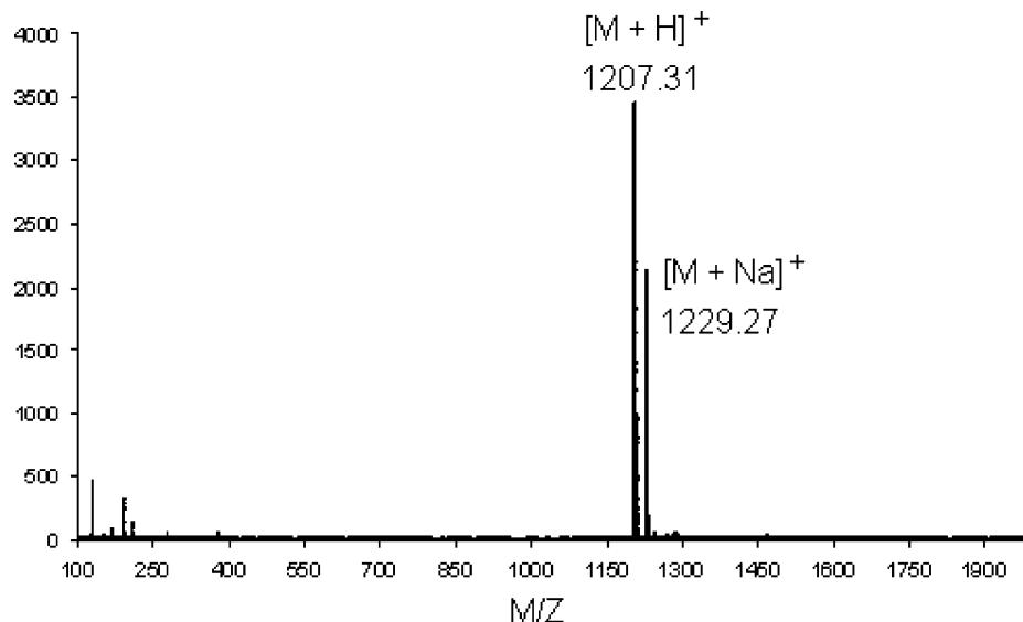
FIGURE 2. MALDI-TOF MS spectra of the G1-NH 2 dendrimer 8 .
