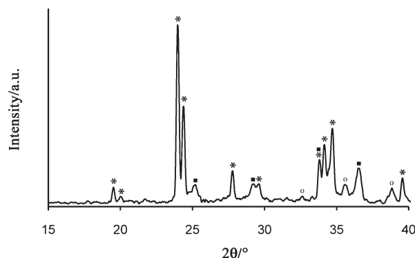
Figure 2. XRD spectrum of a mixture containing \text{Y}(\text{OAc})_3 , \text{Ba}(\text{OAc})_2 , and \text{Cu}(\text{OAc})_2 combusted at 450\text{ }^\circ\text{C} in air for 24 h (■) \text{Y}_2\text{O}_3 (*) \text{BaCO}_3 and (o) CuO.
