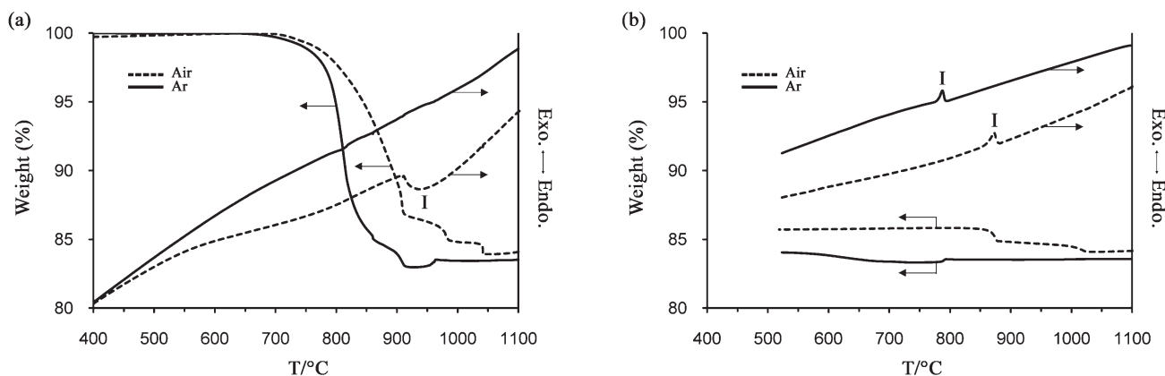
Figure 7. TGA-DTA spectra of a binary mixture of \text{BaCO}_3 and \text{CuO} ( \text{Ba}/\text{Cu} = 2:3 ) in air and Ar when (a) heated at 1\text{ }^\circ\text{C min}^{-1} and (b) cooled at 20\text{ }^\circ\text{C min}^{-1} .
