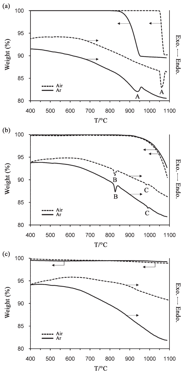
Figure 3. TGA-DTA spectra heated at 10\text{ }^{\circ}\text{C min}^{-1} in air and Ar for (a) CuO, (b) BaCO 3 , and (c) Y 2 O 3 .
