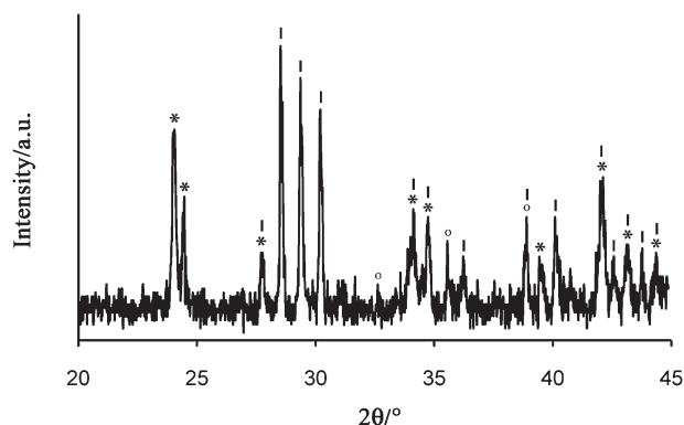
Figure 8. XRD spectrum of a \text{BaCO}_3\text{:CuO} mixture heated at 1000\text{ }^\circ\text{C} for 1 h in \text{N}_2 , (*) \text{BaCO}_3 , (o) \text{CuO} , and (|) \text{BaCuO}_2 .
