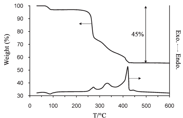
Figure 1. TGA-DTA spectrum in air for a mixture containing \text{Y}(\text{OAc})_3 , \text{Ba}(\text{OAc})_2 , and \text{Cu}(\text{OAc})_2 ( \text{Y}/\text{Ba}/\text{Cu} = 1:2:3 ) heated at 10\text{ }^\circ\text{C min}^{-1} .
