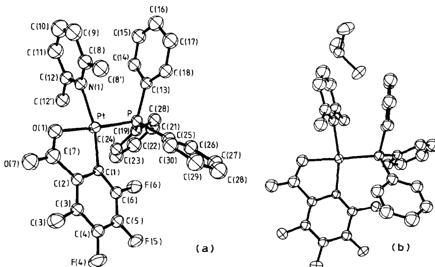
Fig. 1. The crystal structure of \text{Pt}[\text{C}_6\text{F}_4\text{-}o\text{-C(O)O}](\text{PPh}_3)(2,6\text{-Me}_2\text{C}_5\text{H}_3\text{N}) \cdot \text{CHCl}_3 ( 1c · CHCl 3 ). (a) A view showing the numbering of the atoms. Chloroform is omitted for clarity. (b) A view showing chloroform of solvation and the relative positions of the 2,6-dimethylpyridine ligand and the C(13)–C(18) ring of triphenylphosphine.
