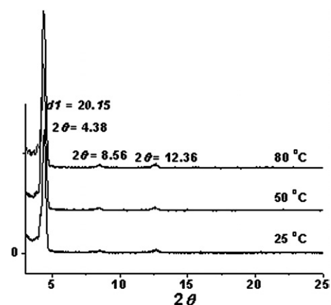
Fig. 4 XRD patterns of DPV-BTBT thin films vacuum-deposited on OTS-treated \text{SiO}_2/\text{Si} at T_{\text{sub}} = 25 , 50 , and 80^{\circ}\text{C} .
