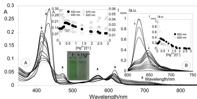
Figure 4. Spectrophotometric (A) and spectrofluorimetric (B) titration of compound \text{1}^- with the addition of \text{Hg}^{2+} in toluene. The inset represents the absorption (A) and the emission intensity (B) as a function of [\text{Hg}^{2+}]/[\text{1}^-] at 420 nm, 440 nm, 575 nm, and 620 nm for (A), and 626 and 650 nm for (B). ( [\text{1}^-] = 9.0 \times 10^{-6} M, \lambda_{\text{exc}} = 565 nm, T = 298 K).
