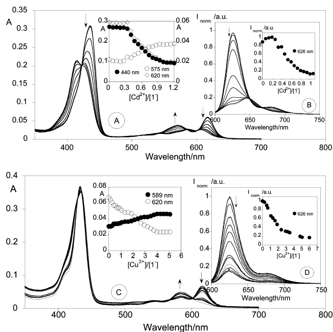
Figure 3. Spectrophotometric (A, C) and spectrofluorimetric (B, D) titration of \text{1}^- with the addition of \text{Cd}^{2+} (A, B) and \text{Cu}^{2+} (C, D) in toluene. The inset represents the absorption at 440 nm, 575 nm, and 620 nm for A, at 589 nm and 620 nm for C; and the emission intensity at 626 nm (B, D) as a function of [\text{Cd}^{2+}]/[\text{1}^-] , and [\text{Cu}^{2+}]/[\text{1}^-] , respectively. ( [\text{1}^-] = 1 \times 10^{-5} M for [\text{Cd}^{2+}] and [\text{1}^-] = 1.2 \times 10^{-5} M for [\text{Cu}^{2+}] , \lambda_{\text{exc}} = 565 nm, T = 298 K).
