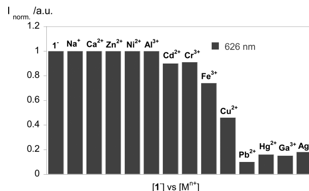
Figure 5. Normalized fluorescence at 626 nm of compound 1 with the first addition of \text{OH}^- (species 1^- ), and after addition of 0.5 equiv of [ \text{M}^{n+} = \text{Na}^+ , \text{Ca}^{2+} , \text{Ni}^{2+} , \text{Zn}^{2+} , \text{Cd}^{2+} , \text{Cu}^{2+} , \text{Pb}^{2+} , \text{Hg}^{2+} , \text{Ga}^{3+} , \text{Cr}^{3+} , \text{Fe}^{3+} , \text{Ag}^+ , and \text{Al}^{3+} ] = \text{M}^{n+} metal ions in toluene.
