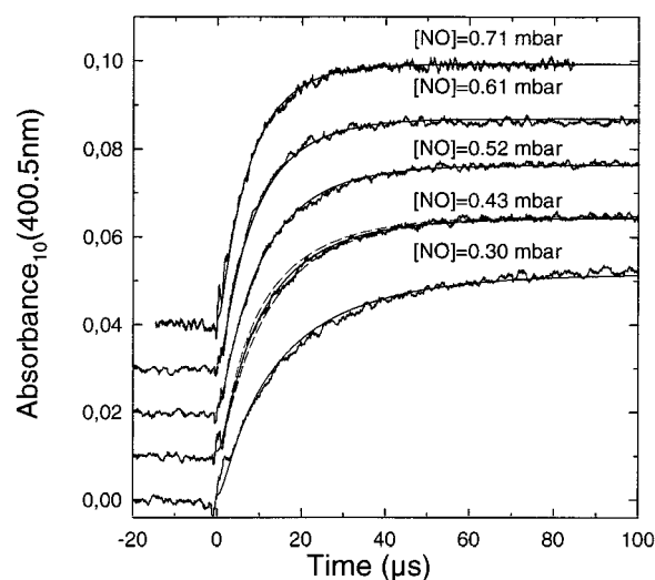
Figure 2. Absorption transients at 400.5 nm following pulsed radiolysis of mixtures of 0.30–0.71 mbar NO, 50 mbar O 2 , 75–100 mbar CH 3 CHO, and 850–875 mbar CO 2 (single pulses, full dose, and optical path length of 120 cm). For clarity, the transients are separated vertically by 0.01 units. The smooth solid lines are simulations using k_2 = 2 \times 10^{-11} \text{ cm}^3 \text{ molecule}^{-1} \text{ s}^{-1} . Additional simulations of the transient where [\text{NO}]_0 = 0.43 \text{ mbar} using k_2 = 1.7 \times 10^{-11} and 2.3 \times 10^{-11} \text{ cm}^3 \text{ molecule}^{-1} \text{ s}^{-1} are shown with smooth dashed lines.
