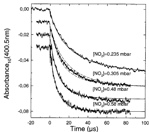
Figure 3. Absorption transients obtained at 400.5 nm following pulsed radiolysis of mixtures of 0.235–0.58 mbar NO 2 , 50 mbar O 2 , 100 mbar CH 3 CHO, and 850 mbar CO 2 (single pulses, full dose, and optical path length of 120 cm). The smooth solid lines are simulations using k_3 = 1 \times 10^{-11} cm 3 molecule -1 s -1 . Additional simulations of the transient where [\text{NO}_2]_0 = 0.305 mbar using k_3 = 0.8 \times 10^{-11} and 1.2 \times 10^{-11} cm 3 molecule -1 s -1 are shown with smooth dashed lines.
