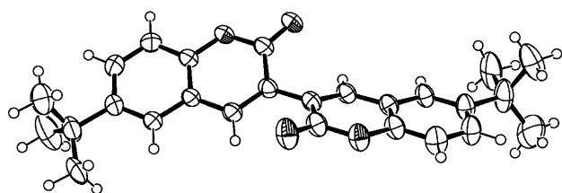
Figure 1. Solid-state molecular structure of 6,6'-di-tert-butyl-2H,2'H-3,3'-bichromen-2,2'-dione 3a . Thermal ellipsoids are set at 50% probability. For clarity, the disordered tert -butyl groups are shown in one conformation only. [19]
