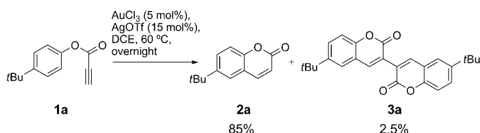
Scheme 1. Formation of dicoumarins in the Au-catalyzed cyclization of aryl propargylesters (DCE = 1,2-dichloroethane).
