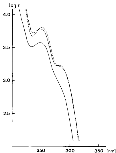
Fig. 1. Long-wavelength part of the electronic-absorption spectra of (\pm)\text{-4} (—), (\pm)\text{-trans-7} (---), and (\pm)\text{-cis-7} (-.-) in EtOH
