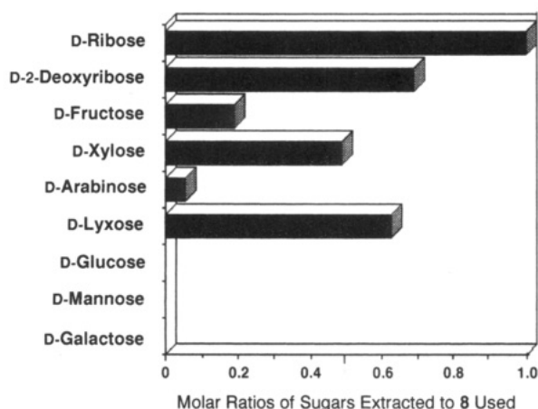
Figure 6. Extractabilities of various sugars with 8 . For details, see Experimental Section.
