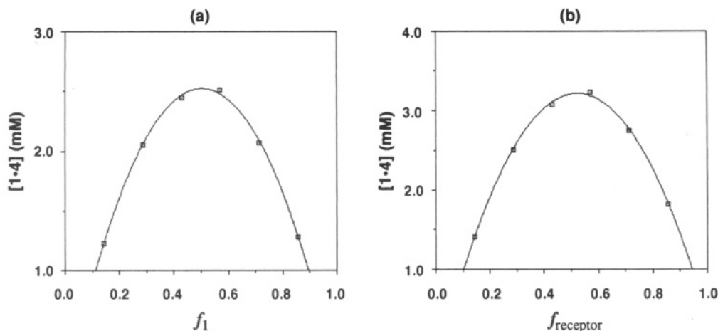
Figure 2. Job's plots of [complex] vs mole fractions of (a) 1 ( f_1 ) and (b) 4 ( f_{\text{receptor}} ) for the complexation of 1 and 4 in \text{CDCl}_3 at 23 °C. For details, see Experimental Section.
