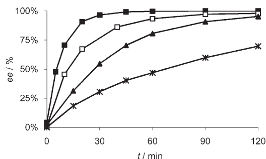
Figure 3. Enantiomeric excesses for the HKR of epichlorohydrin at 0.5 mol %: 4b (■), homogeneous \text{Co}^{\text{III}} –salen (□), 4a (▲), and 7 (*).
