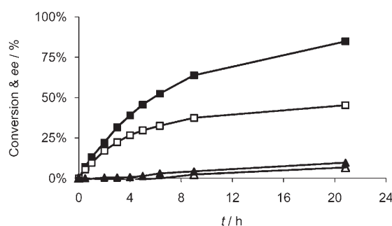
Figure 2. Kinetic data for the HKR of epichlorohydrin at 0.01 mol %: 4b ee (■), 4b conversion (□), homogeneous \text{Co}^{\text{III}} –salen ee (▲), and homogeneous \text{Co}^{\text{III}} –salen conversion (△).
