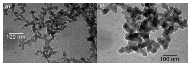
Figure 1. TEM images at 100,000× of a) CAB-O-SIL silica and b) polymer brush 3b .
