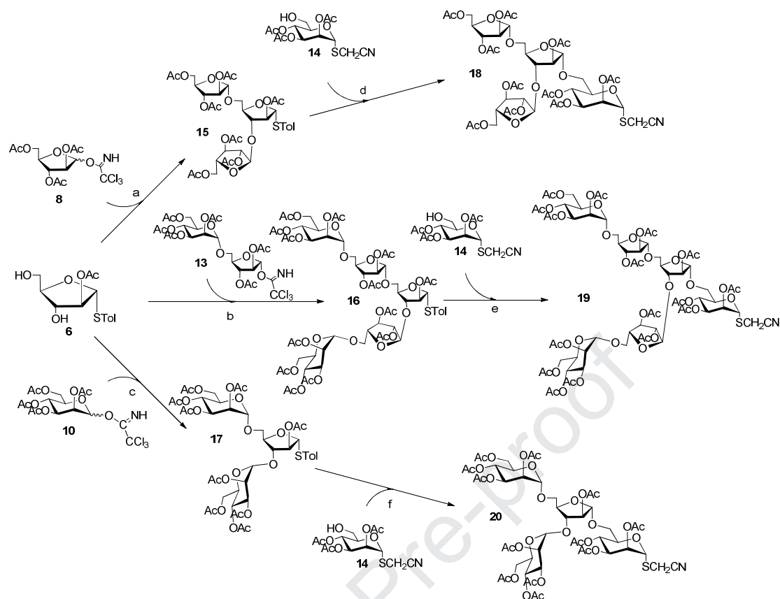
Scheme 3. Reagents and conditions: (a) \text{BF}_3 \cdot \text{Et}_2\text{O} , 4 Å MS, \text{CH}_2\text{Cl}_2 , 0 °C, 30 min, 40%; (b) \text{BF}_3 \cdot \text{Et}_2\text{O} , 4 Å MS, \text{CH}_2\text{Cl}_2 , 0 °C, 1 h, 32%; (c) \text{BF}_3 \cdot \text{Et}_2\text{O} , 4 Å MS, \text{CH}_2\text{Cl}_2 , 0 °C, 1 h, 37%; (d) NIS, AgOTf, 4 Å MS, \text{CH}_2\text{Cl}_2 , -30 °C, 50 min, 60%; (e) NIS, AgOTf, 4 Å MS, \text{CH}_2\text{Cl}_2 , -30 °C, 50 min, 49%; (f) NIS, AgOTf, 4 Å MS, \text{CH}_2\text{Cl}_2 , -30 °C, 50 min, 55%
