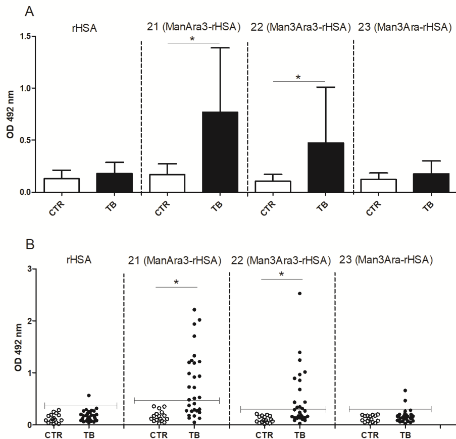
Figure 4. Antibodies (IgG) levels reactive against neoglycoproteins 21 , 22 and 23 in 30 TB patients and 16 healthy subjects (CTR).
