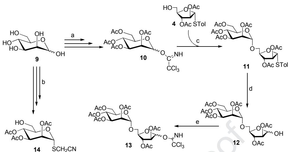
Scheme 2. Reagents and conditions: Transformations (a) and (b) have been conducted using reported protocols[23,28]; (c) \text{BF}_3 \cdot \text{Et}_2\text{O} , 4 Å MS, \text{CH}_2\text{Cl}_2 , -60\text{ }^\circ\text{C} , 30 min, 55%; (d) NIS, AgOTf, TTBP, wet \text{CH}_2\text{Cl}_2 , 0\text{ }^\circ\text{C} - RT, 1 h, 90%; (e) \text{CCl}_3\text{CN} , DBU, \text{CH}_2\text{Cl}_2 , 0\text{ }^\circ\text{C} , 30 min, 90%.
