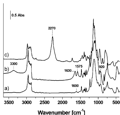
Figure 1. IR spectra in KBr matrix of a) Ti-NH 2 POSS, b) Ti-POSS-TSIP (2) and c) 3-isocyanatopropyl triethoxysilane.
