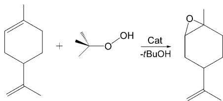
Scheme 2. Limonene (1-methyl-4-(prop-1-en-2-yl)cyclohex-1-ene) epoxidation with TBHP.
