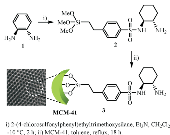
Scheme 1 Preparation of the MCM-41-supported chiral ligand 3
