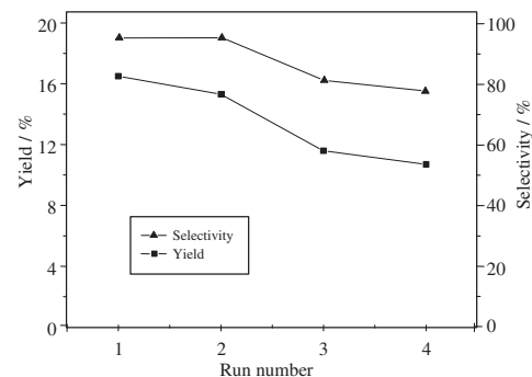
Figure 4. Reusage of CoMnNi/SiO 2 catalyst.
