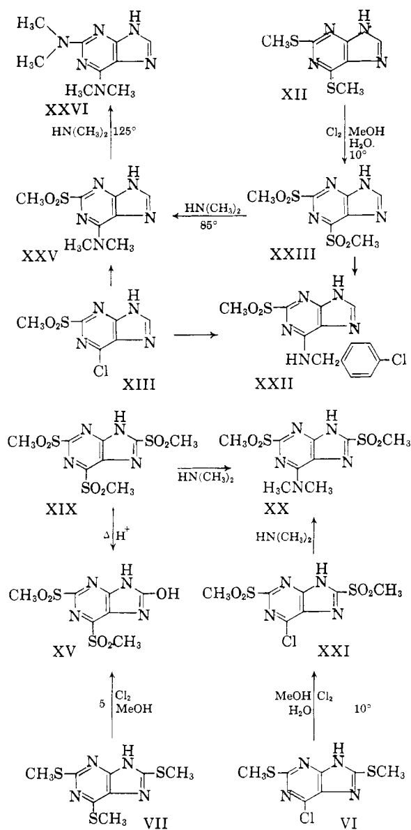
REACTION SCHEME IV
