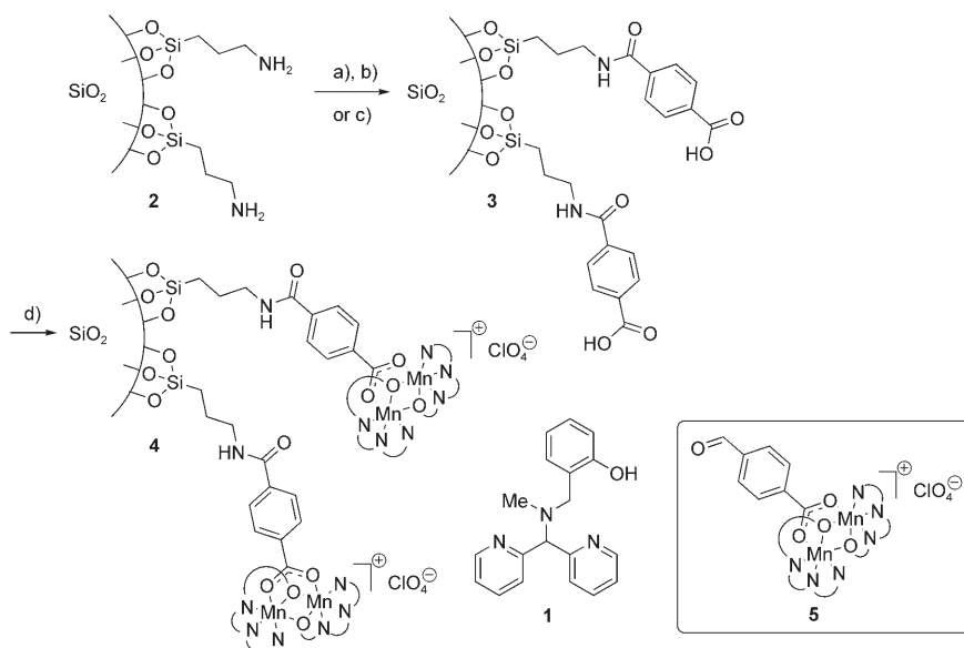
Scheme 3. Synthesis of surface bound manganese catalyst anchored via an amide linkage. a) Methyl 4-(chlorocarbonyl)benzoate, \text{Et}_3\text{N} , toluene; b) KOH, \text{H}_2\text{O} , EtOH; terephthalic acid, DCC, DMAP, toluene; d) \text{Mn}(\text{ClO}_4)_2 , \text{Et}_3\text{N} , 1 , MeOH, MeCN.
