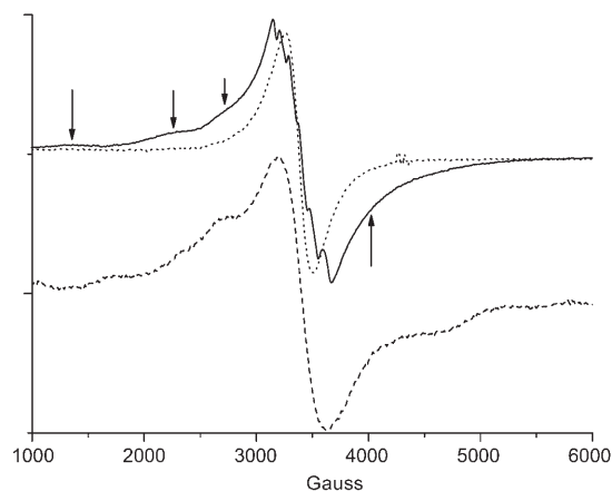
Figure 2. EPR spectra (X-band at 77 K) of —: silica supported manganese catalyst 16 (suspension in DCM), ----: non-bound manganese catalyst 5 (2.10 -3 M in DCM) and .....: ligand free silica supported Mn II . Recording conditions: microwave power = 63.5 mW; modulation amplitude = 0.1 mT; modulation frequency = 50 kHz; time constant = 40.96 ms; T = 77 K at 9.47 GHz.
