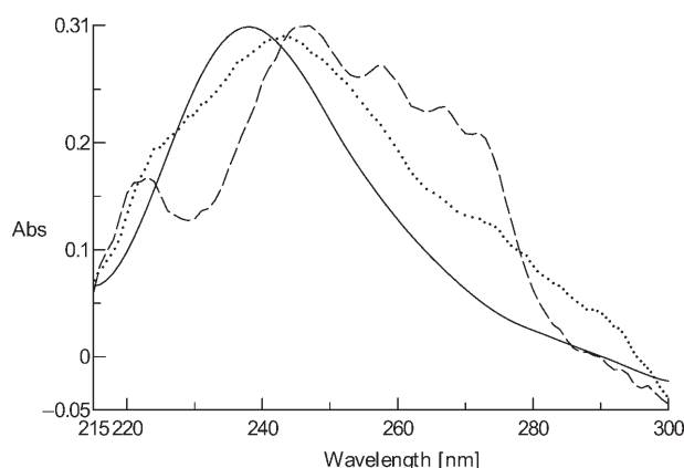
Figure 1. UV/Vis spectra of —: amide tethered benzoic ester 11 (2.10 -5 M in CH 3 CN), ----: non-bound manganese catalyst 5 (2.10 -5 M in CH 3 CN) and .....: silica supported manganese catalyst 16 (DR UV/Vis, suspension in glycerol).
