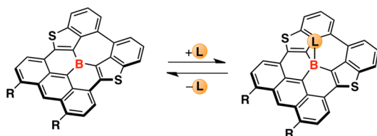
Scheme 2. Interconversion between 5 and the Corresponding Borate by Reaction with a Lewis Base
