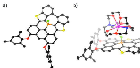
Figure 5. X-ray crystal structure of 5 ·F – [K(cryptand)] + (50% probability for thermal ellipsoids). (a) Top view, in which [K(cryptand)] + was omitted for clarity, and (b) side view.
