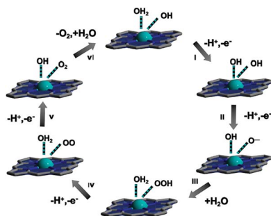
Scheme 1 Proposed reaction mechanism of Cu-CNTCPP for OER.
