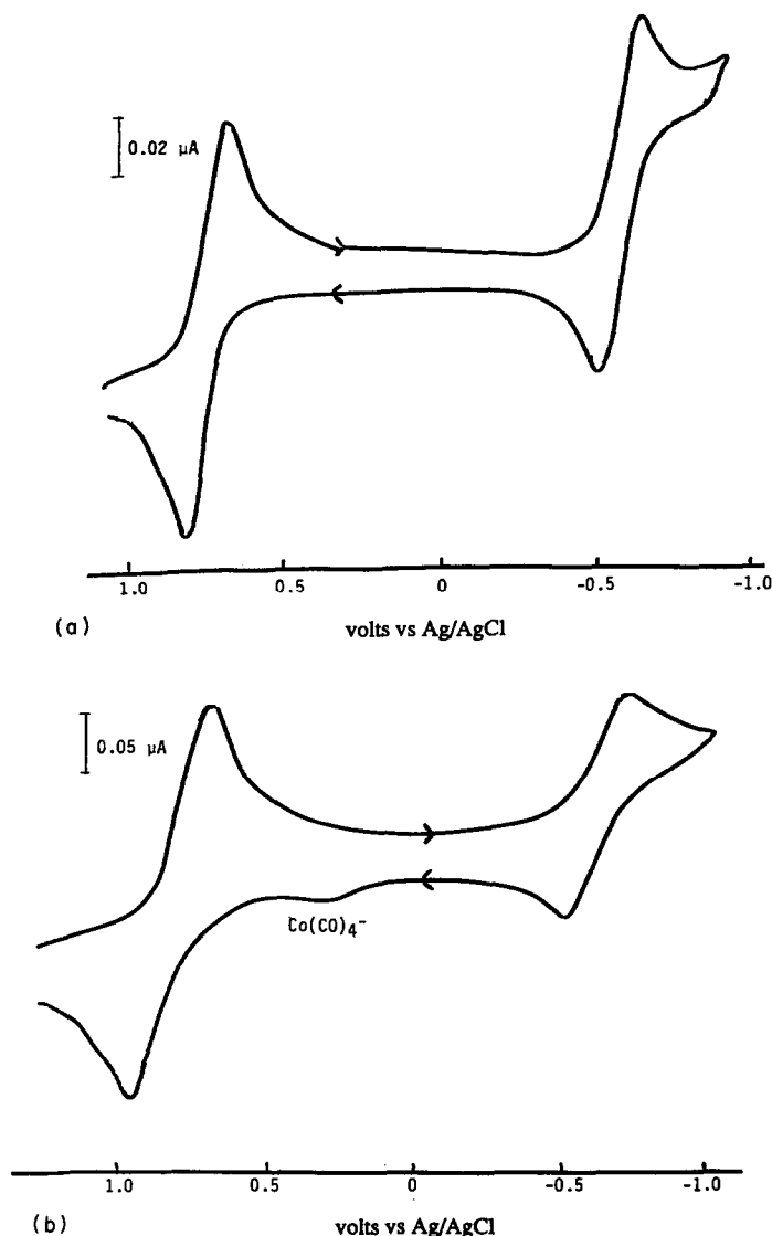
Fig. 2. Cyclic voltammogram in \text{CH}_2\text{Cl}_2 under Ar (295 K) at Pt. (a) 1a : 50 \text{ mV s}^{-1} ; (b) 1b : 200 \text{ mV s}^{-1} .
