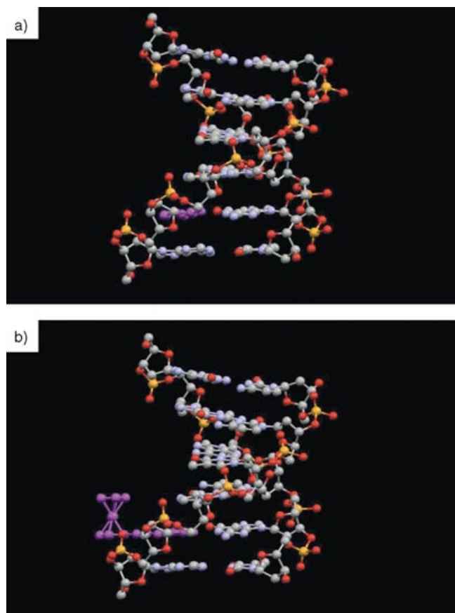
Figure 5. Gas-phase PM3-optimised structures of 6-mer duplexes AC x GTCC, with a) C x =cytidine and b) C x =C5-ethynylferrocenyl-cytidine, showing co-planarity of ferrocene and cytidine ring.
