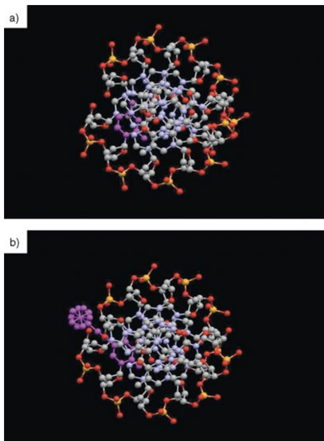
Figure 6. 6-mer duplexes of AC x GTCC, with a) C x =cytidine and b) C x =C5-ethynylferrocenyl-cytidine, viewed along the helical axis, showing the ferrocene moiety sitting external to the phosphate backbone in the major groove.
