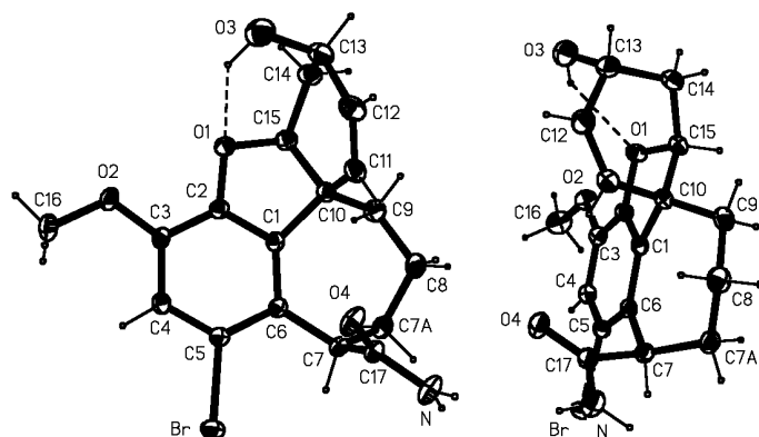
Figure 2. Molecular structure of 11 in crystalline 11 \cdot \frac{1}{2} \text{C}_2\text{H}_5\text{OH} (20% ellipsoids) seen in two views (crystallographic atom numbering).
