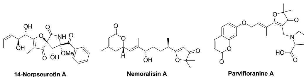
Figure 1. Naturally occurring products containing the 3(2H)-furanone skeleton.
