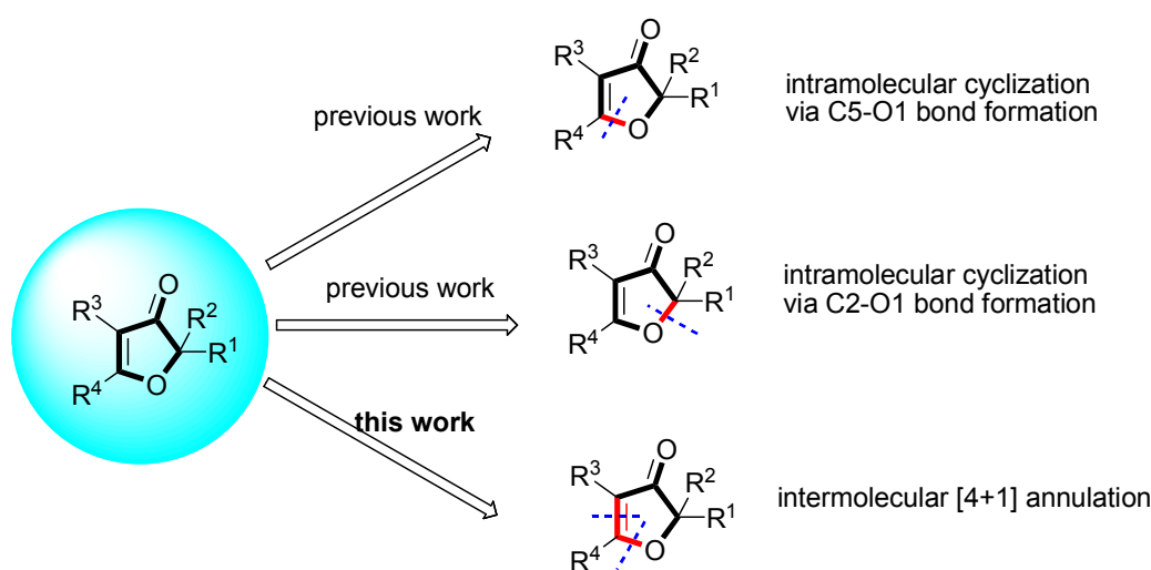
Figure 2. Synthetic Strategies to 3(2 H )-furanones.
