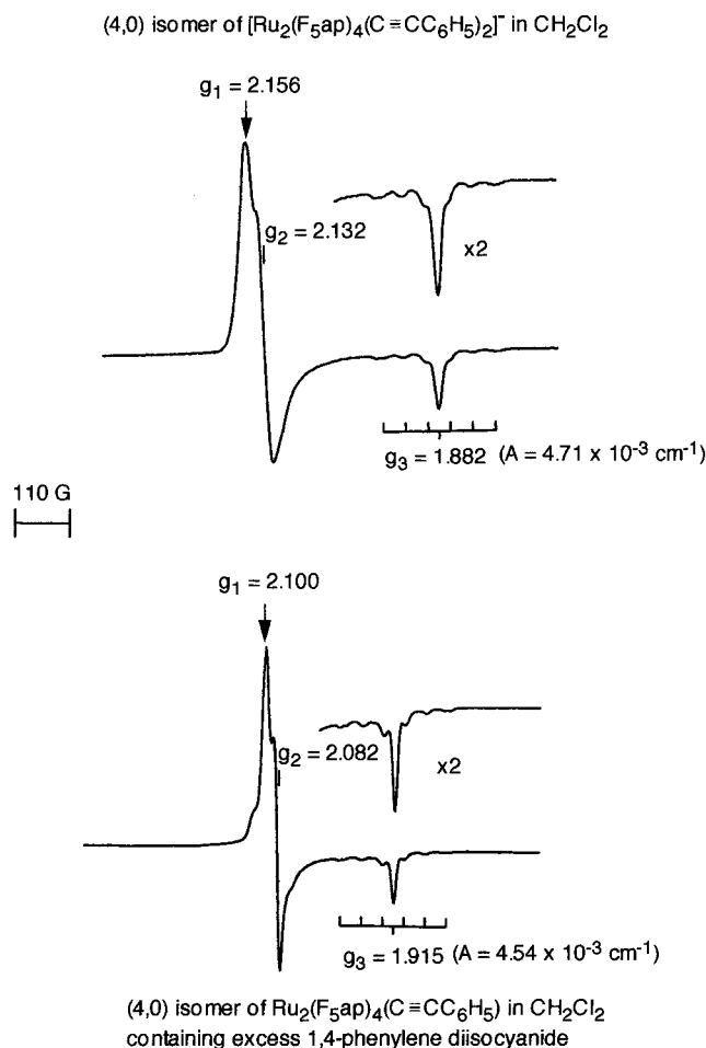
Figure 5. ESR spectra (77 K) of the electrogenerated (4,0) isomer of [Ru 2 (F 5 ap) 4 (C≡CC 6 H 5 ) 2 ] •− in CH 2 Cl 2 , 0.1 M TBAP and Ru 2 (F 5 ap) 4 (C≡CC 6 H 5 ) in CH 2 Cl 2 containing excess 1,4-phenylene diisocyanide.
