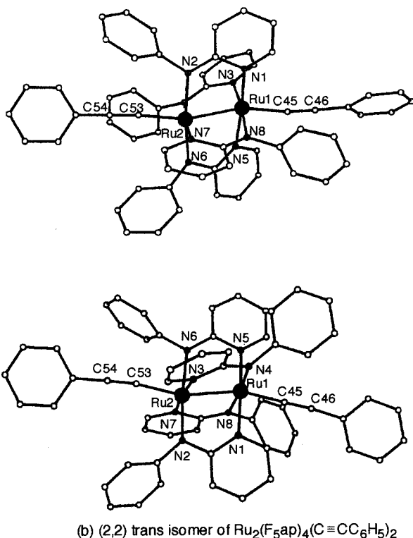
Figure 2. Views of (a) the (3,1) isomer and (b) the (2,2) trans isomer of \text{Ru}_2(\text{F}_5\text{ap})_4(\text{C}\equiv\text{CC}_6\text{H}_5)_2 with H and F atoms omitted.
