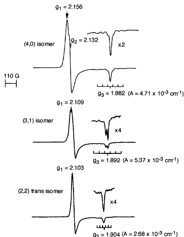
Figure 4. ESR spectra (77 K) in CH 2 Cl 2 , 0.2 M TBAP of the electrogenerated (4,0), (3,1), and (2,2) trans isomers of [Ru 2 (F 5 ap) 4 (C≡CC 6 H 5 ) 2 ] •− .
