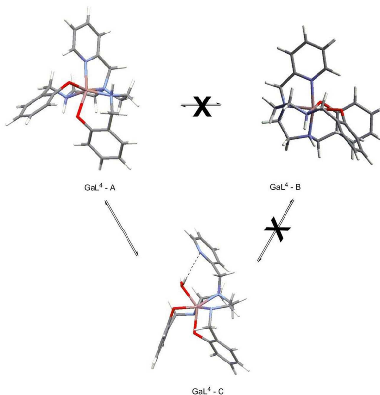
Scheme 3: [\text{GaL}^{\text{py,NH}}]^+ species present in acetonitrile solution.
