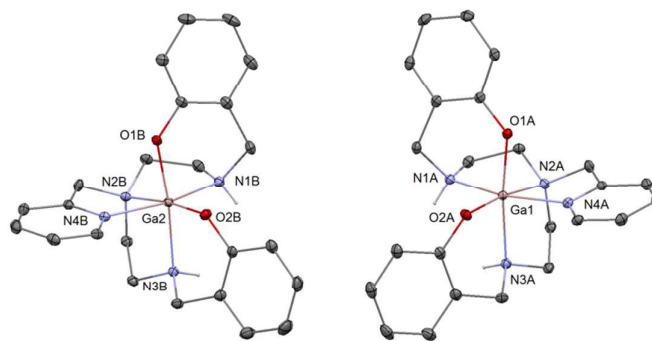
Figure 2. ORTEP drawing at the 40% probability level for the two enantiomers of [\text{GaL}^{\text{py,NH}}]^+ cation in [\text{GaL}^{\text{py,NH}}]\text{ClO}_4 . Hydrogen atoms are omitted for clarity with exception of those attached to the coordinating aliphatic amine groups.
