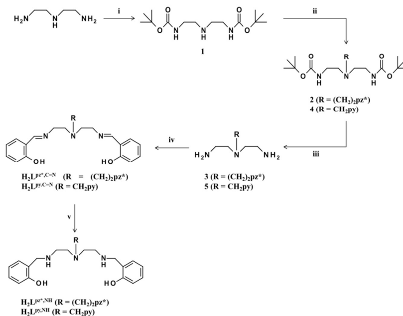
Scheme 1. Synthesis of the ligands. i) \text{O}(\text{BOC})_2 , THF, r.t., o.n.; ii) \text{BrCH}_2\text{CH}_2(3,5\text{-Me}_2\text{pz}) or 2\text{-BrCH}_2\text{py} , \text{K}_2\text{CO}_3 , KI, THF, reflux, 24 h; iii) \text{HCl}/\text{MeOH} , r.t., 2 h; iv) salicylaldehyde, \text{MeOH} , reflux, 4 h; v) \text{NaBH}_4 , \text{MeOH} , r.t., o.n.
