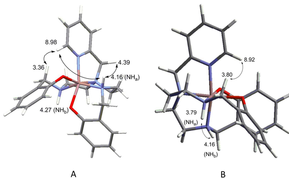
Figure 5. Relevant NOE enhancements used to confirm the mer -N3dien coordination in isomer A and the fac -N3dien coordination in isomer B of [\text{GaL}^{\text{py,NH}}]^+ in \text{CD}_3\text{CN} .
