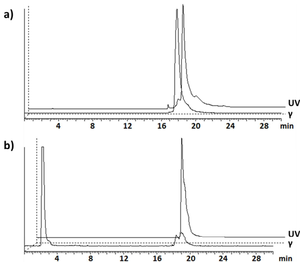
Figure 7. HPLC chromatograms of: a) [\text{GaL}^{\text{py},\text{NH}}](\text{ClO}_4) (UV detection) and reaction mixture of the radiolabeling of \text{H}_2\text{L}^{\text{py},\text{NH}} with ^{67}\text{GaCl}_3 ( \gamma detection); b) [\text{GaL}^{\text{pz}^*,\text{NH}}](\text{ClO}_4) (UV detection) and reaction mixture of the radiolabeling of \text{H}_2\text{L}^{\text{pz}^*,\text{NH}} with ^{67}\text{GaCl}_3 ( \gamma detection).
