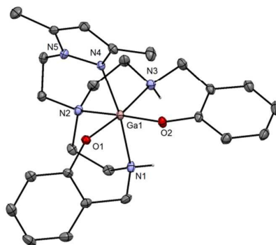
Figure 1. ORTEP drawing at the 40% probability level for the [\text{GaL}^{\text{pz}^*,\text{NH}}]^+ cation in [\text{GaL}^{\text{pz}^*,\text{NH}}]\text{ClO}_4 . Hydrogen atoms are omitted for clarity with exception of those attached to the coordinating aliphatic amine groups.
