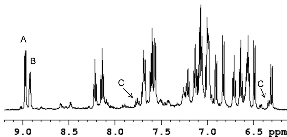
Figure 4. Aromatic region of the ^1\text{H} spectrum of [\text{GaL}^{\text{py},\text{NH}}]^+ in \text{CD}_3\text{CN} showing the presence of two major isomers A and B in a 1:0.6 ratio. Some of the peaks of the minor species C are also identified.
