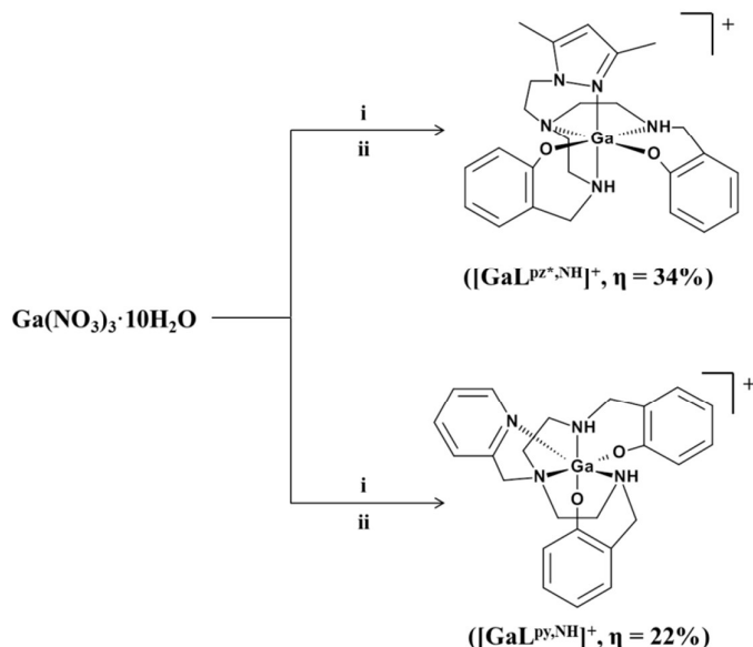
Scheme 2. Synthesis of the gallium complexes. i) \text{H}_2\text{L}^{\text{pz}^*,\text{NH}} or \text{H}_2\text{L}^{\text{py},\text{NH}} , \text{NaCH}_3\text{COO} , \text{MeOH} , r.t., o.n.; ii) \text{NaClO}_4 .
