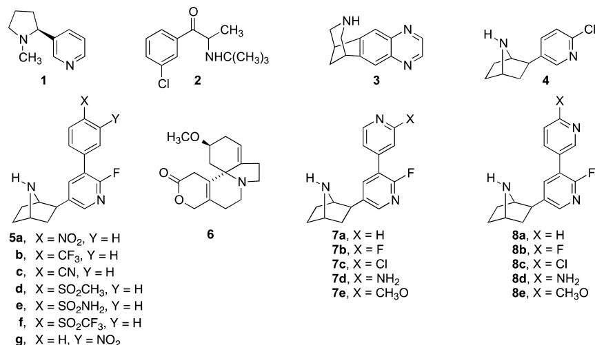
Chart 1. Structures of Compounds 1–4, 5a–g, 6, 7a–e, and 8a–e
