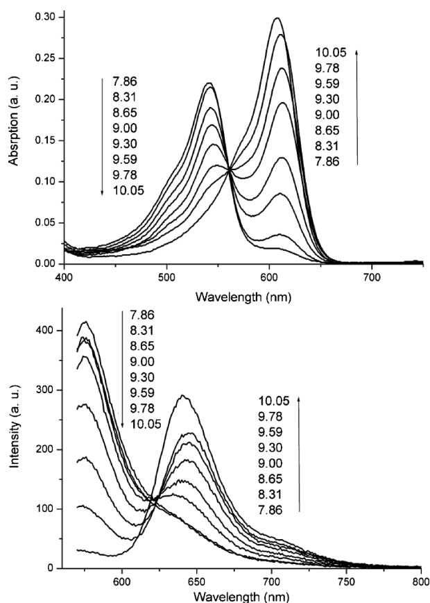
Fig. 1 Absorption spectra (top) of BODIPY-OH in buffer solution as a function of pH. Corresponding emission spectra (bottom) ( \lambda_{\text{ex}} = 559 nm). pH was adjusted by \text{NaH}_2\text{PO}_4 and \text{Na}_2\text{HPO}_4 .
