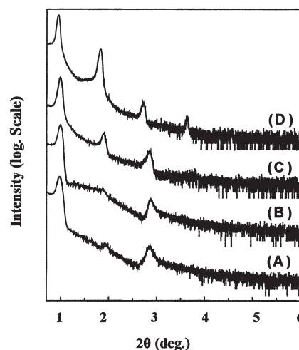
Figure 1. Small-angle XRD patterns corresponding to a lamellar-to-hexagonal phase transformation in mesostructured silica thin films synthesized using \text{EO}_{20}\text{PO}_{70}\text{EO}_{20} surfactant. The sample was heated under a water vapor hydrothermal condition, where the temperature was ramped at a rate of 1 °C/min from 25 °C (trac A), to 80 °C (trace B), 110 °C (trace C), and 150 °C (trace D), respectively.
