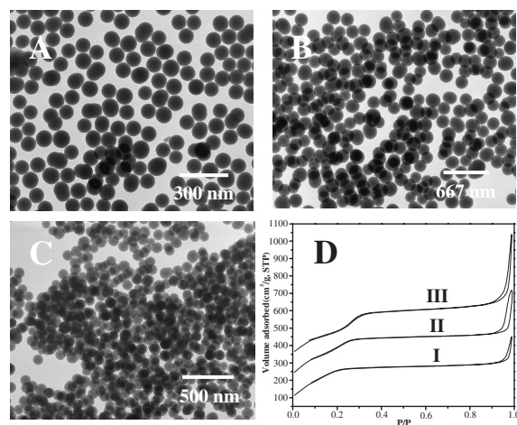
Figure 1. The TEM images and N 2 adsorption–desorption isotherms of the mesoporous silica spheres synthesized from C_n TMAB–sodium silicate–H 2 O–ethanol components at different pH value. A. C_{12} TMAB, ethanol/H 2 O = 0 g/ 275 g, pH = 8.0, the sphere size = 155 \pm 15 nm. B. C_{14} TMAB, ethanol/H 2 O = 70 g/275 g, pH = 8.0, the sphere size = 173 \pm 17 nm. C. C_{16} TMAB, ethanol/H 2 O = 80 g/275 g, pH = 8.0 the sphere size = 117 \pm 10 nm. D. N 2 adsorption–desorption isotherms of A–C samples. The pore size analyzed by BJH method of sample A = 1.85 nm (I); the pore size of sample B = 2.30 nm (II); the pore size of sample C = 2.52 nm (III).
