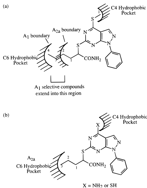
Figure 2. Hypothetical C-4 and C-6 hydrophobic pockets of adenosine A 1 and A 2a receptors. The combined C-4/C-6 hydrophobic pocket tolerance of alkyl carbons: (a) at the A 1 receptor, five, one at C-4 and four at C-6; at the A 2a receptor, three, one at C-4 and two at C-6 (for the methylthio substituent) or, alternatively, (b) at the A 2a receptor, three, zero at C-4 and three at C-6 (for the mercapto or amino substituent).
