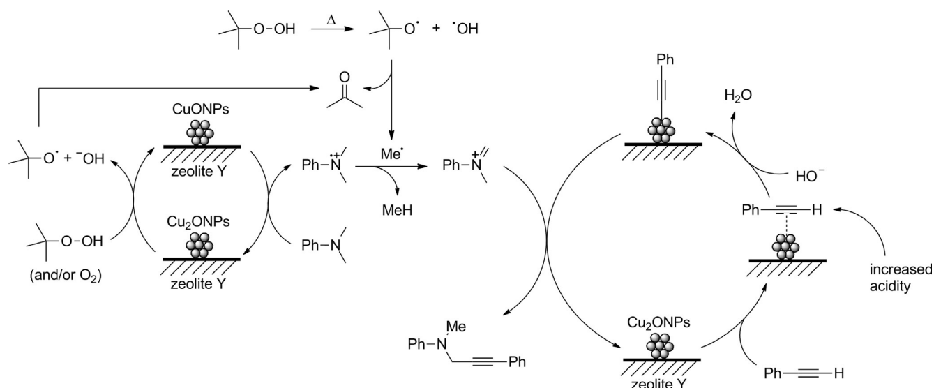
Scheme 7. Reaction mechanism proposed for the CDC of N,N -dimethylaniline and phenylacetylene catalyzed by CuNPs/ZY in the presence of TBHP.
