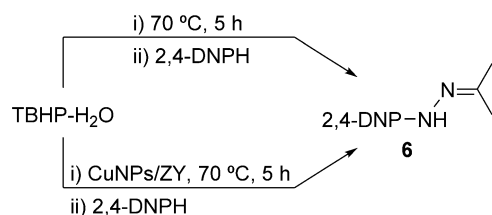
Scheme 5. Control experiments on the transformation of TBHP into acetone.
