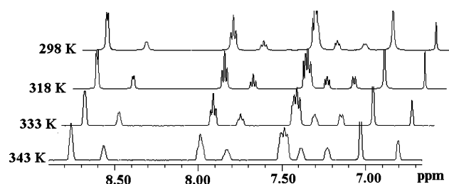
Fig. 2 1 H NMR spectra of the aromatic region for [Zn 2 (CH 3 L2)(CH 3 -COO) 2 ](PF 6 ) in CD 3 CN at four different temperatures.
