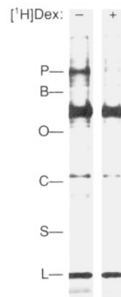
Figure 3. Fluorograph of [ 3 H]Dex-NCS-labeled HTC cell receptors. A 50% solution of HTC cell cytosol in pH 7.5 HEPES buffer was incubated with 3.1 \times 10^{-7} M [ 3 H]Dex-NCS ± 30-fold excess unlabeled Dex for 2.5 h at 0 °C. An aliquot was mixed with an equal volume of 2× SDS sample buffer at room temperature and then electrophoresed on an SDS-polyacrylamide gel (10.5%). The above fluorograph of the dried gel was obtained after a 13 day exposure of the film.
