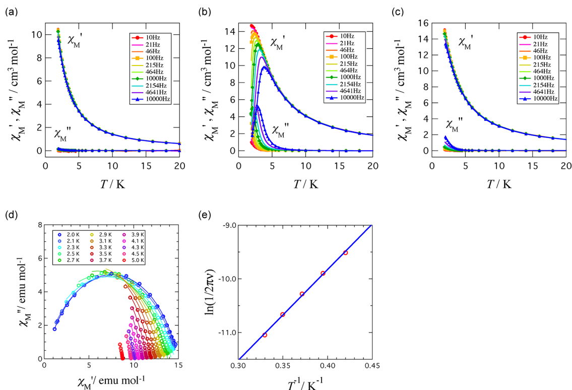
Figure 12. Plots of the in-phase ( \chi_M' ) and out-of-phase ( \chi_M'' ) ac susceptibility of (a) the Co II –Gd III , (b) Co II –Tb III , and (c) Co II –Dy III complexes measured at a dc bias field of 1000 Oe, (d) Cole–Cole plot, and (e) Arrhenius plot of the Co II –Tb III complex.
