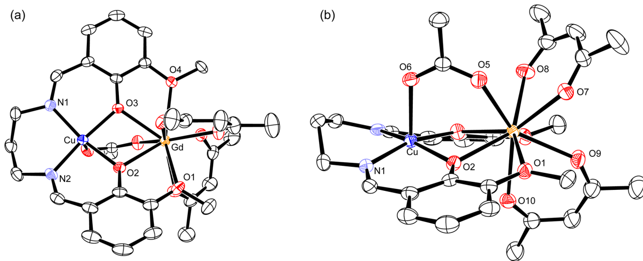
Figure 1. Molecular structure of acetato- and diphenolato-bridged binuclear \text{Cu}^{\text{II}}\text{--Gd}^{\text{III}} complex with the selected atom numbering scheme. The hydrogen and fluorine atoms are omitted for clarity. (a) Perspective view projected on equatorial \text{N}_2\text{O}_2 plane. (b) Side view showing acetato-bridge.
