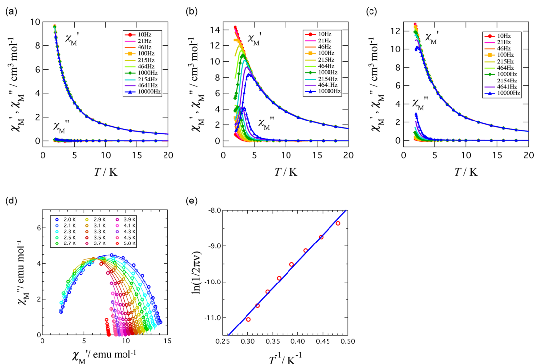
Figure 11. Plots of the in-phase ( \chi_M' ) and out-of-phase ( \chi_M'' ) ac susceptibility of (a) the \text{Ni}^{\text{II}}-\text{Gd}^{\text{III}} , (b) \text{Ni}^{\text{II}}-\text{Tb}^{\text{III}} , and (c) \text{Ni}^{\text{II}}-\text{Dy}^{\text{III}} complexes measured at a dc bias field of 1000 Oe, (d) Cole–Cole plot, and (e) Arrhenius plot of the \text{Ni}^{\text{II}}-\text{Tb}^{\text{III}} complex.
