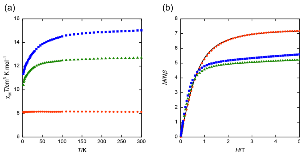
Figure 3. (a) Plots of \chi_M T vs T for binuclear \text{Zn}^{\text{II}}\text{--Ln}^{\text{III}} complexes [ \text{Ln}^{\text{III}} = \text{Gd}^{\text{III}} (red), \text{Tb}^{\text{III}} (green), and \text{Dy}^{\text{III}} (blue)]. (b) Field dependence of the magnetization for the \text{Zn}^{\text{II}}\text{--Ln}^{\text{III}} complexes [ \text{Ln}^{\text{III}} = \text{Gd}^{\text{III}} (red), \text{Tb}^{\text{III}} (green), and \text{Dy}^{\text{III}} (blue)] at 1.9 K, as plots of M/N\beta vs H . The solid line of the \text{Zn}^{\text{II}}\text{--Gd}^{\text{III}} complex represents the theoretical curve of M = Ng\beta S_B(y) for g = 2.06 and S = 7/2 .
