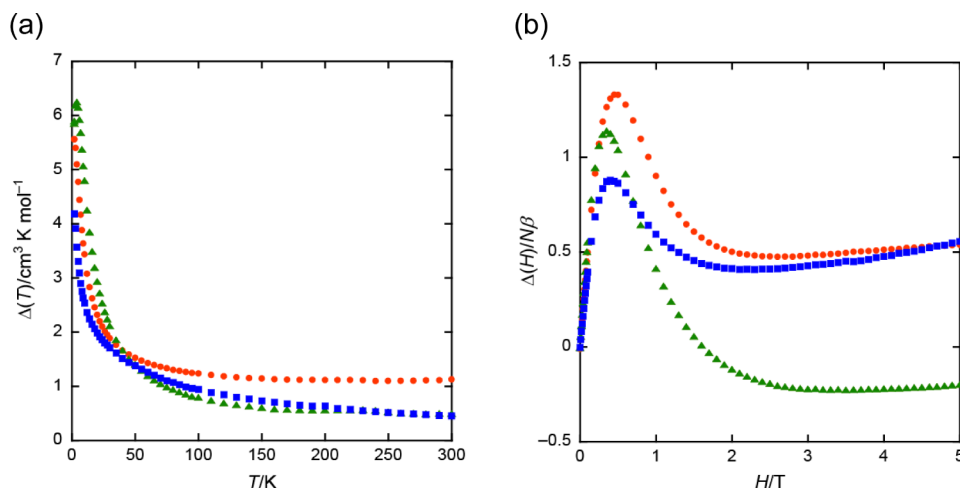
Figure 9. (a) Plots of \Delta(T) = (\chi_M T)_{\text{CoLn}} - (\chi_M T)_{\text{CoLa}} - (\chi_M T)_{\text{ZnLn}} vs temperature T for the \text{Co}^{\text{II}}\text{--Ln}^{\text{III}} complexes [ \text{Ln}^{\text{III}} = \text{Gd}^{\text{III}} (red), \text{Tb}^{\text{III}} (green), and \text{Dy}^{\text{III}} (blue)]. (b) Plots of \Delta(H) = M_{\text{CoLn}}(H) - M_{\text{CoLa}}(H) - M_{\text{ZnLn}}(H) vs H for the \text{Co}^{\text{II}}\text{--Ln}^{\text{III}} complexes [ \text{Ln}^{\text{III}} = \text{Gd}^{\text{III}} (red), \text{Tb}^{\text{III}} (green), and \text{Dy}^{\text{III}} (blue)].
