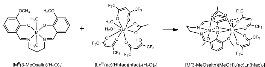
Scheme 1. Synthetic Scheme of Acetato- and Diphenolato-Bridged Binuclear 3d–4f Complex, [\text{M}(\text{3-MeOsalt})_x(\text{MeOH})_x(\text{ac})\text{Ln}(\text{hfac})_2] ( x = 0 for \text{M} = \text{Cu}^{\text{II}} , \text{Zn}^{\text{II}} ; x = 1 for \text{M} = \text{Co}^{\text{II}} , \text{Ni}^{\text{II}} ; \text{Ln} = \text{Gd}^{\text{III}} , \text{Tb}^{\text{III}} , \text{Dy}^{\text{III}} and \text{La}^{\text{III}} ), by the Reaction of [\text{M}(\text{3-MeOsalt})_x(\text{H}_2\text{O})_x] and [\text{Ln}(\text{ac})(\text{Hhfac})(\text{hfac})_2(\text{H}_2\text{O})_2]
