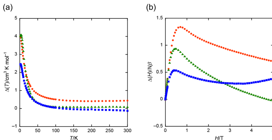
Figure 8. (a) Plots of \Delta\chi_M(T) = (\chi_M T)_{\text{NiLn}} - (\chi_M T)_{\text{ZnLn}} - (\chi_M T)_{\text{NiLa}} vs T for the \text{Ni}^{\text{II}}\text{--Ln}^{\text{III}} complexes [ \text{Ln}^{\text{III}} = \text{Gd}^{\text{III}} (red), \text{Tb}^{\text{III}} (green), and \text{Dy}^{\text{III}} (blue)]. (b) Plots of \Delta(H) = M_{\text{NiLn}}(H) - M_{\text{ZnLn}}(H) - M_{\text{NiLa}}(H) vs H for the \text{Ni}^{\text{II}}\text{--Ln}^{\text{III}} complexes [ \text{Ln}^{\text{III}} = \text{Gd}^{\text{III}} (red), \text{Tb}^{\text{III}} (green), and \text{Dy}^{\text{III}} (blue)].
