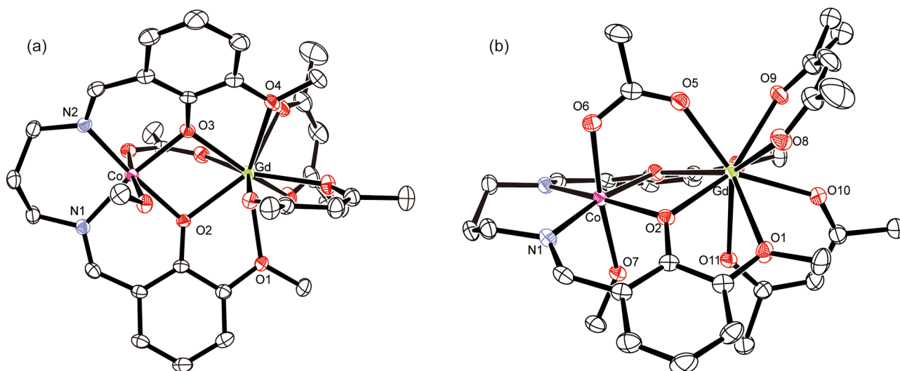
Figure 2. Molecular structure of acetate- and diphenolato-bridged binuclear \text{Co}^{\text{II}}\text{--Gd}^{\text{III}} complex with the selected atom numbering scheme. The \text{Co}^{\text{II}} ion assumes octahedral coordination geometry with equatorial tetradentate ligand and acetate and methanol oxygens. The hydrogen and fluorine atoms and solvent molecule are omitted for clarity. (a) Perspective view projected on equatorial \text{N}_2\text{O}_2 plane. (b) Side view showing acetate-bridge and coordination of methanol to Co.
