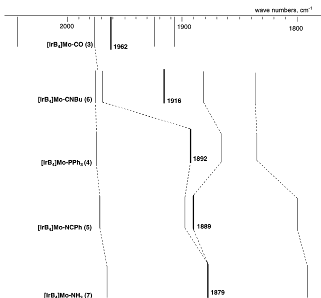
Figure 3. Representation of the IR spectra. The average frequencies are given in boldface type, which for the \text{PPh}_3 , NCPh, and \text{NH}_3 derivatives coincide with one of the spectral bands. The dotted lines do not imply assignments and illustrate only frequency shifts.
