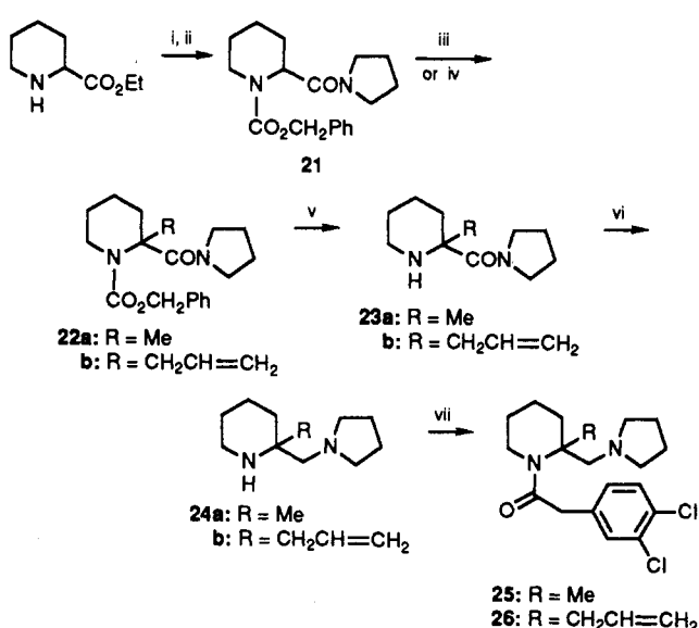
Scheme IV a
