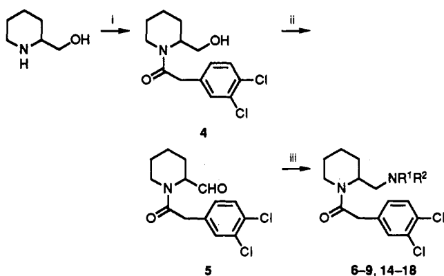
Scheme I a
