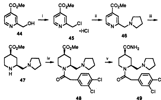
Scheme VII a
