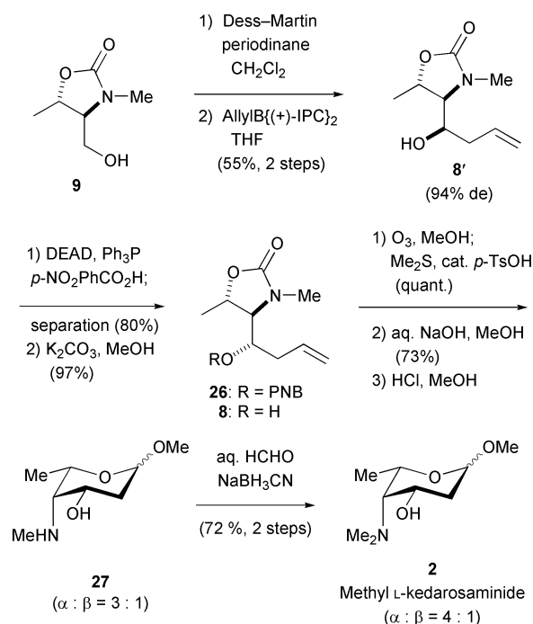
Scheme 7 Synthesis of methyl kedarosaminide.
