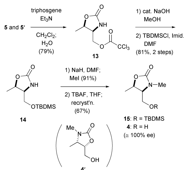
Scheme 2 Introduction of nitrogen functional group.
