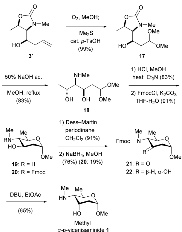
Scheme 4 Synthesis of methyl vicanisaminide.
