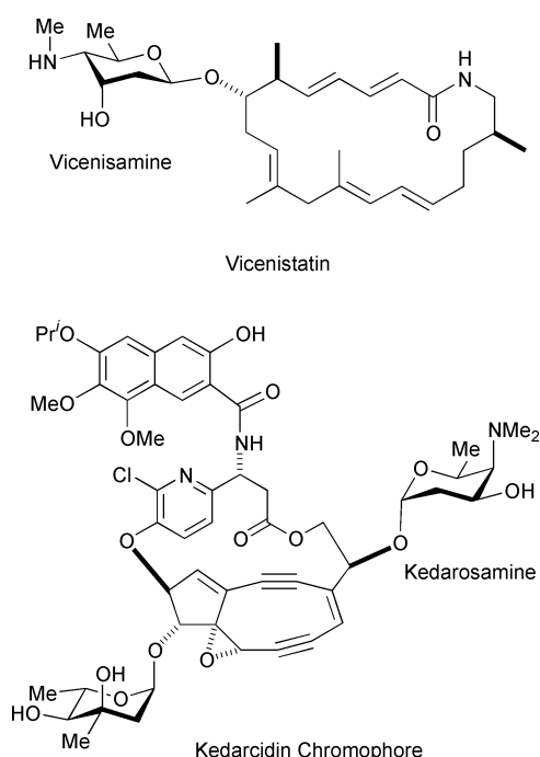
Fig. 1 Structure of vicenistatin and kedaricin chromophore.
