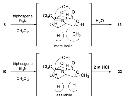
Fig. 2 Lability of intermediary imidatonium ions to hydrolytic conditions.
