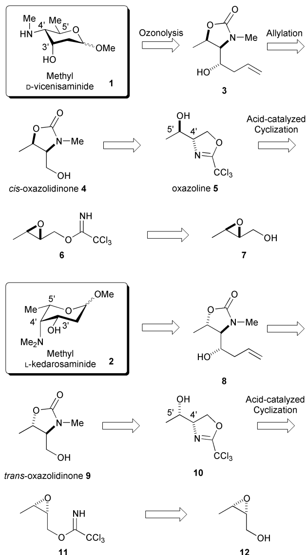
Scheme 1 Retrosynthetic analysis of vicenissamine and kedarosamine.
