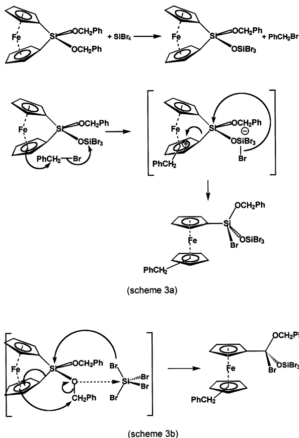
Scheme 3. Formation of T structures in the solid: (a) with release of alkyl halide; (b) concerted process.
