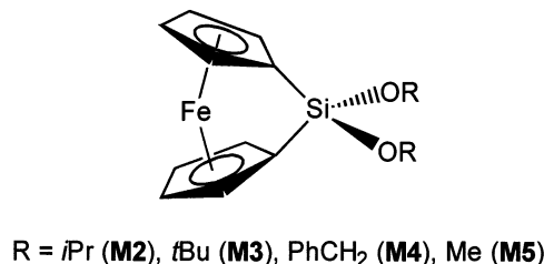
Scheme 2. Monomers M2–M5 .
